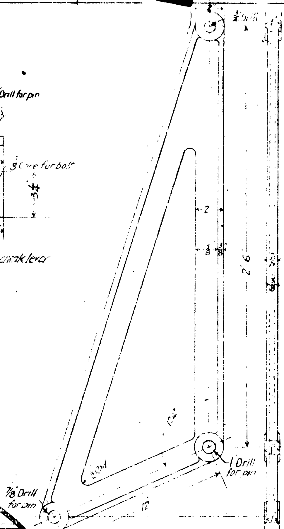
Main Cast Iron Pat. N o 7,349-A 1 Req d
