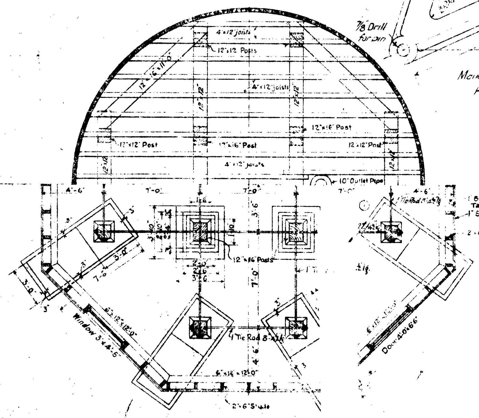
HALF-PLAN OF JOISTS UNDER TANK HALF FOUNDATION PLAN
