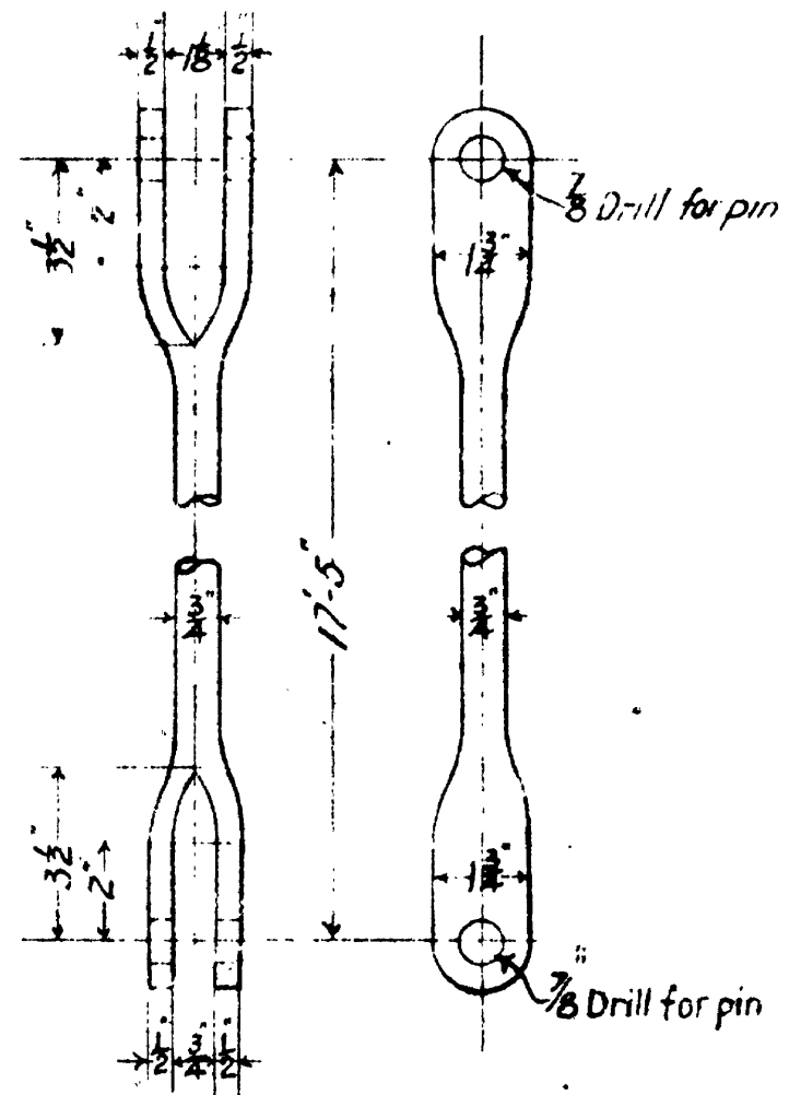
Forged Connecting Rod Bell-crank lever to valve lever 1 Req d
