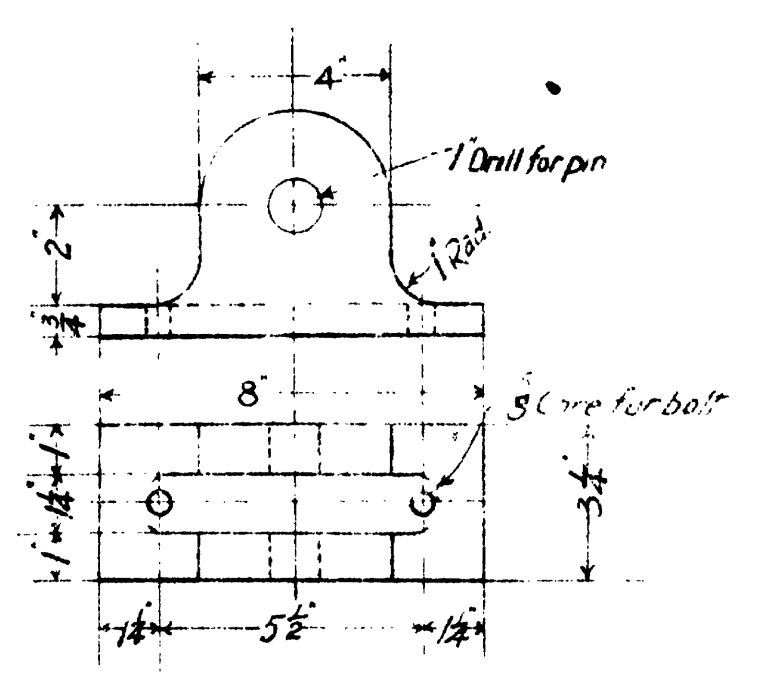
Cast Iron Bracket for Bell-crank lever 1 Req d Pat. N o 7,345
