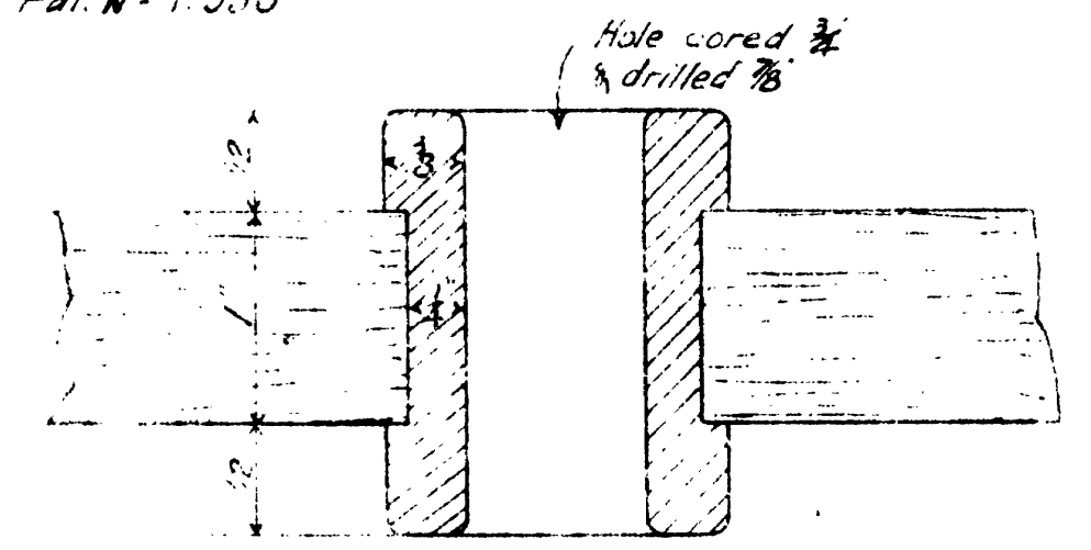
Section C.I. Thimble for Valve Rope - Full Size
