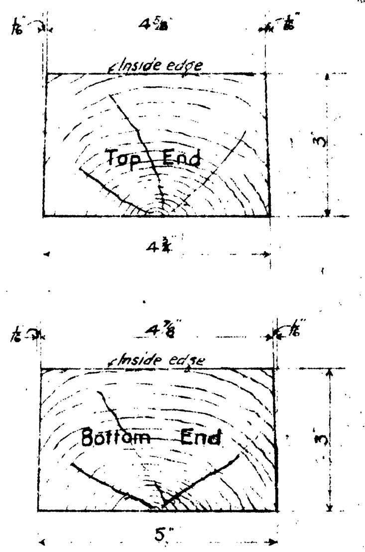
DETAIL OF STAVE HALF FULL SIZE
